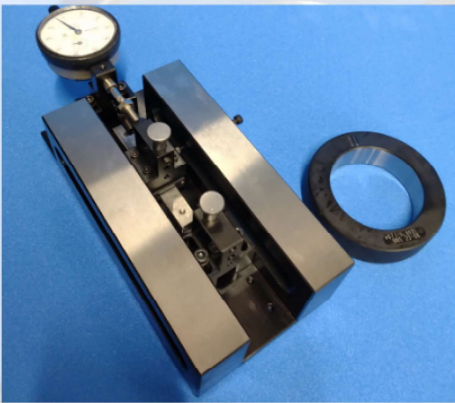
内径測定器 (ASQA-ID-01)
